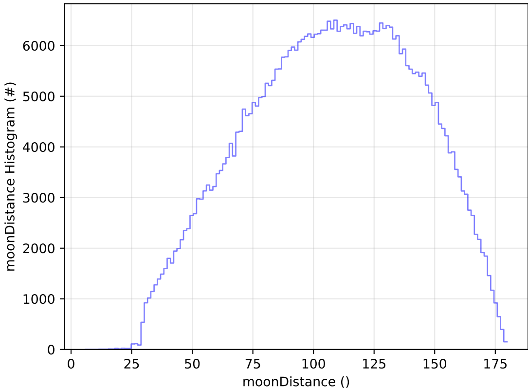
too_combined_s0.5_v3.4_10yrs WFD r band: moonDistance Histogram
