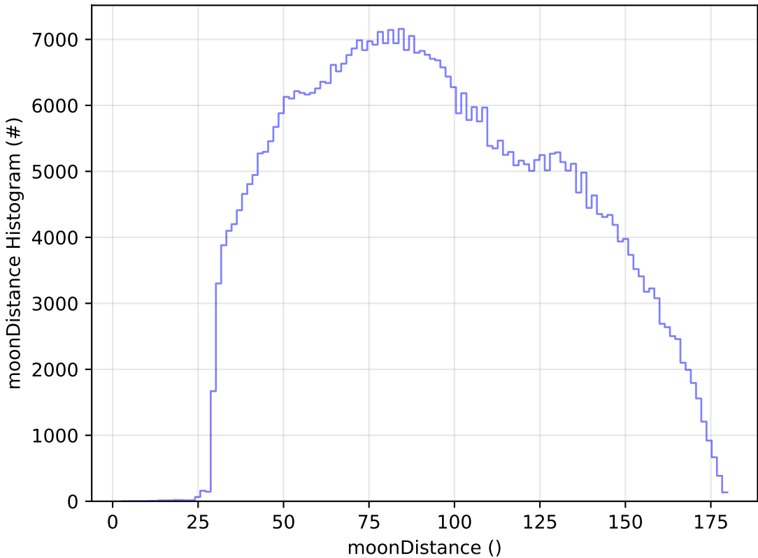
too_combined_s0.5_v3.4_10yrs WFD i band: moonDistance Histogram
