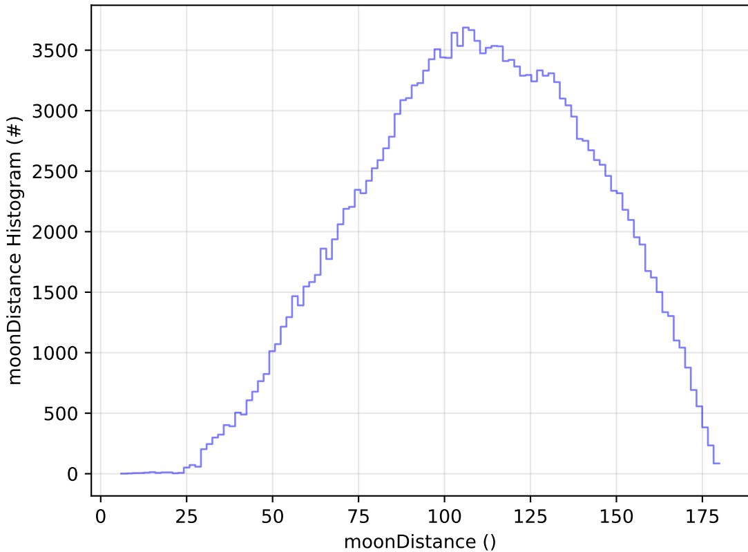
too_combined_s0.5_v3.4_10yrs WFD g band: moonDistance Histogram
