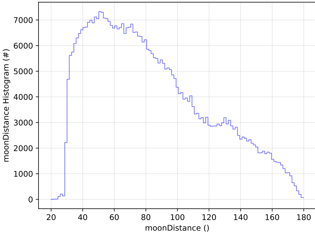
too_combined_s0.5_v3.4_10yrs All sky z band: moonDistance Histogram
