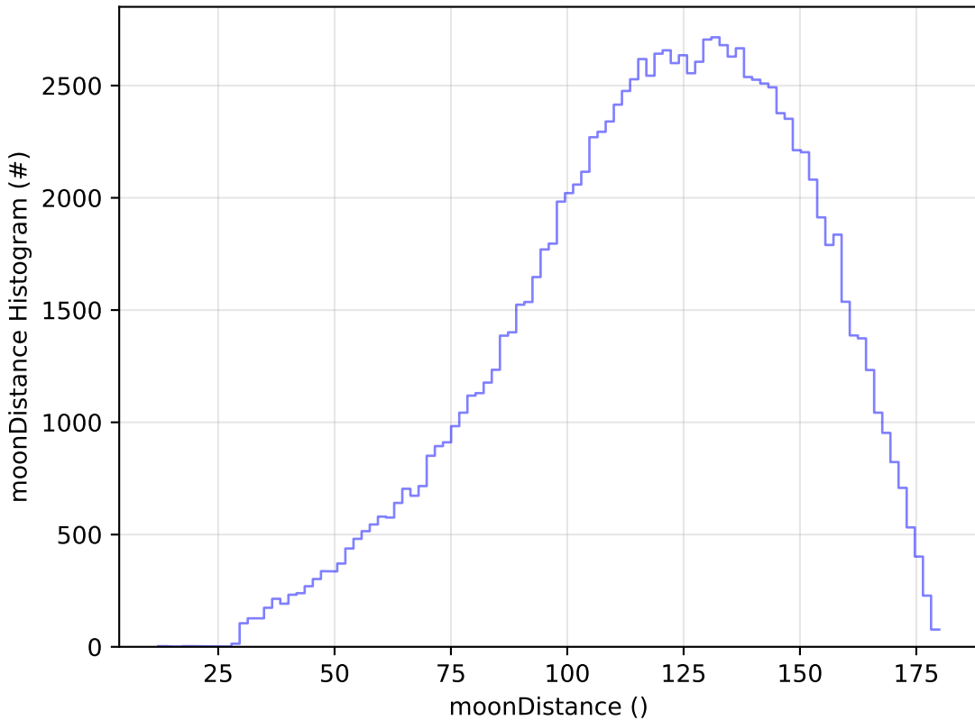
too_combined_s0.5_v3.4_10yrs All sky u band: moonDistance Histogram
