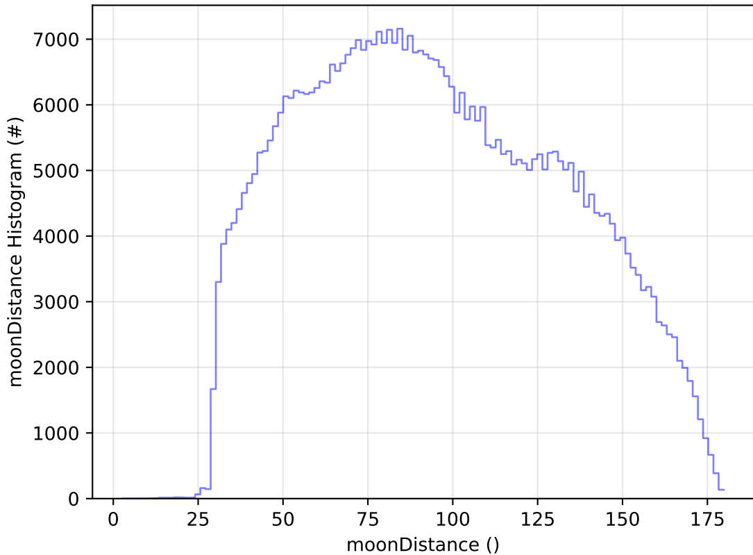
too_combined_s0.5_v3.4_10yrs All sky i band: moonDistance Histogram
