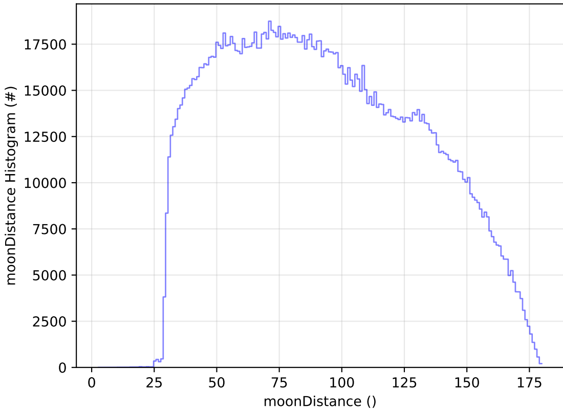
too_combined_s0.5_v3.4_10yrs All sky all bands: moonDistance Histogram
