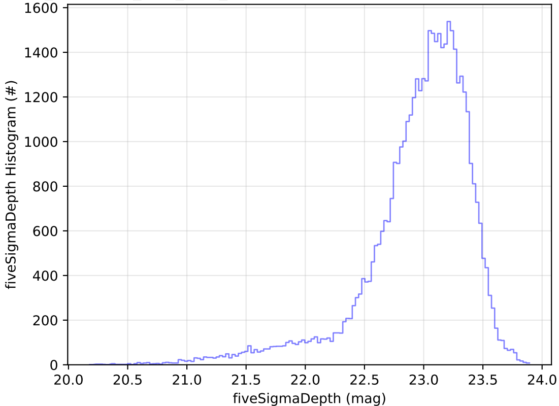
too_combined_s0.5_v3.4_10yrs Yr 1 z band: fiveSigmaDepth Histogram
