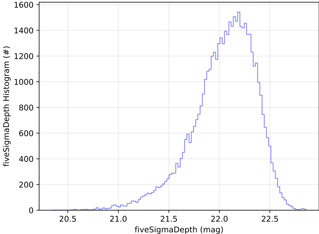
too_combined_s0.5_v3.4_10yrs Yr 1 y band: fiveSigmaDepth Histogram
