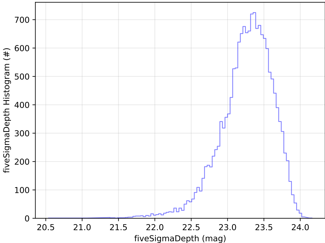
too_combined_s0.5_v3.4_10yrs Yr 1 u band: fiveSigmaDepth Histogram
