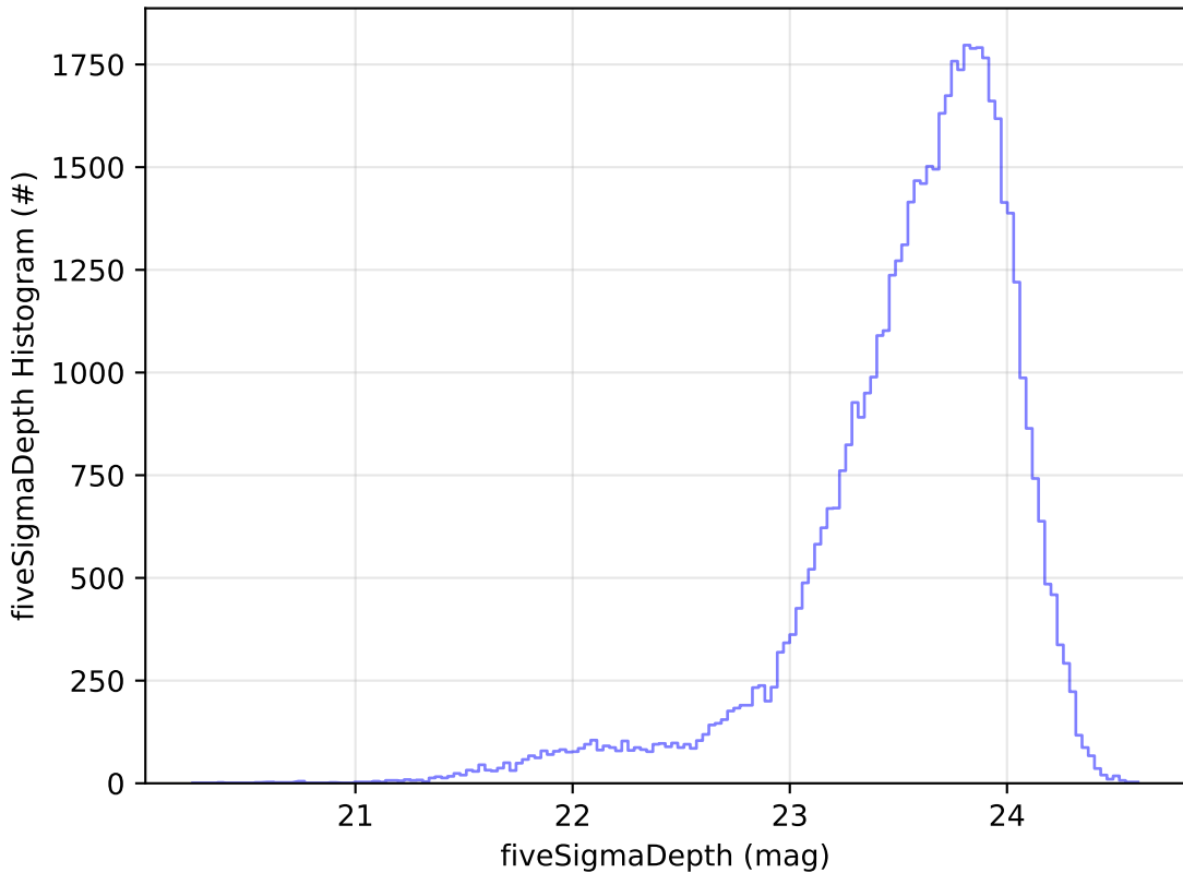
too_combined_s0.5_v3.4_10yrs Yr 1 i band: fiveSigmaDepth Histogram
