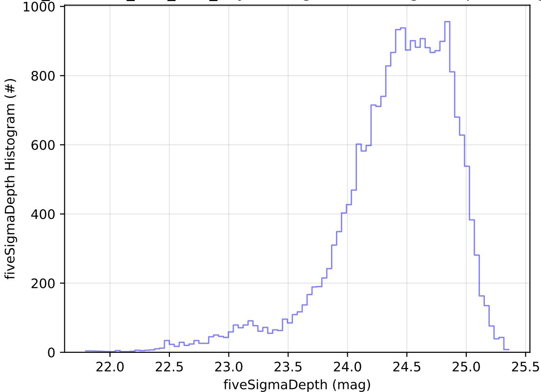
too_combined_s0.5_v3.4_10yrs Yr 1 g band: fiveSigmaDepth Histogram
