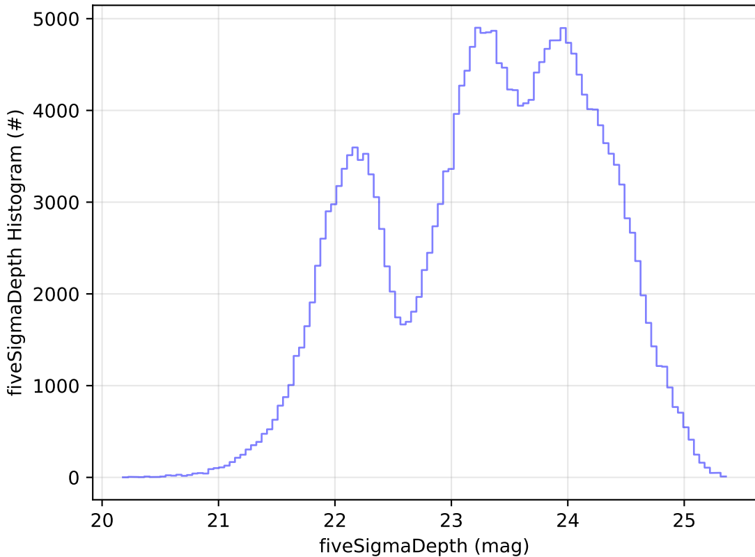
too_combined_s0.5_v3.4_10yrs Yr 1 all bands: fiveSigmaDepth Histogram
