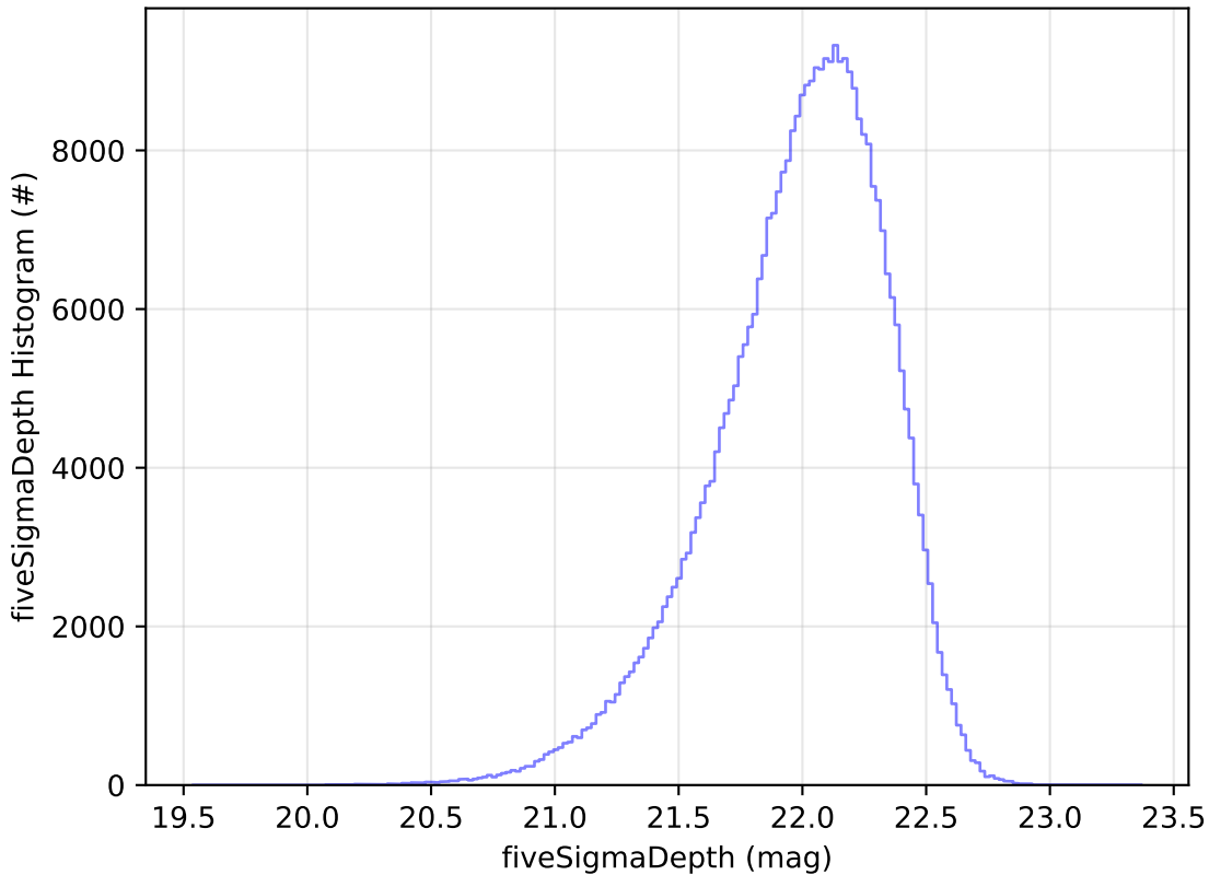
too_combined_s0.5_v3.4_10yrs WFD y band: fiveSigmaDepth Histogram
