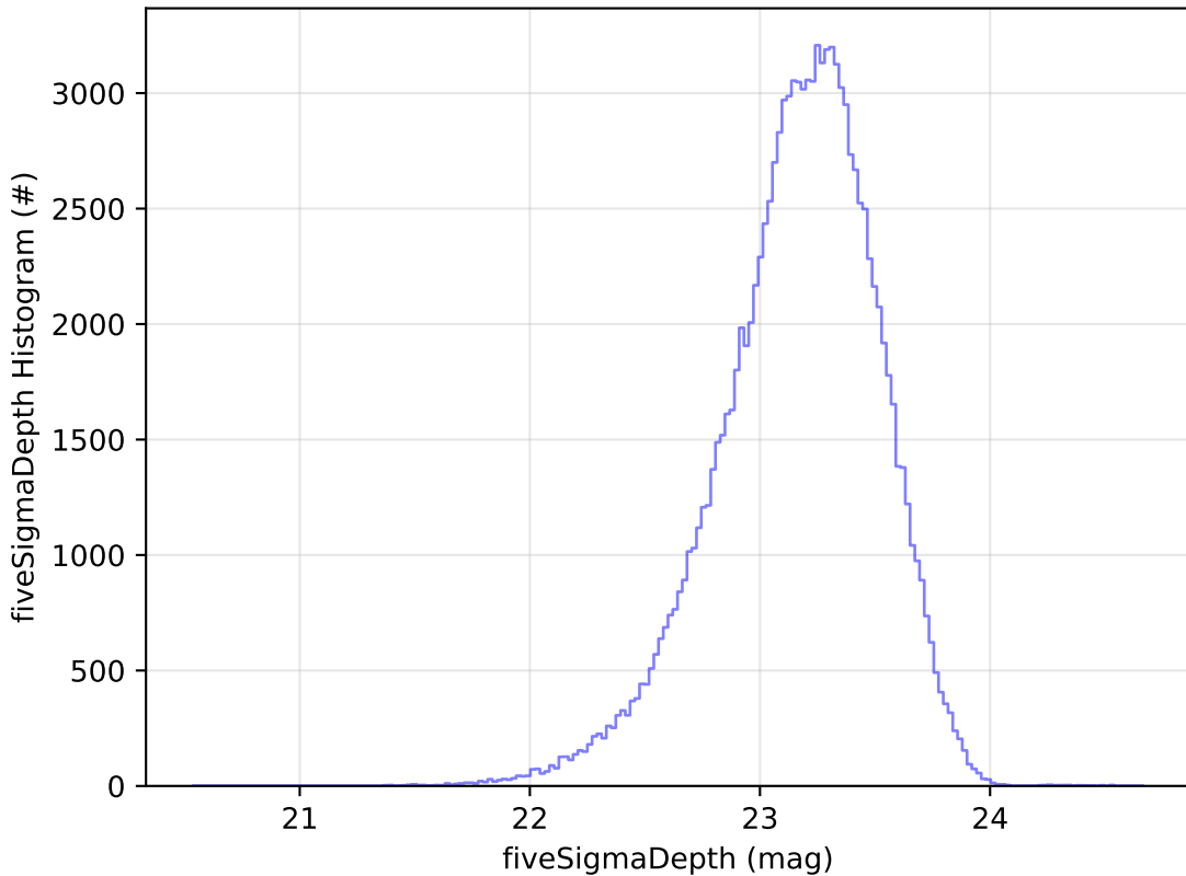
too_combined_s0.5_v3.4_10yrs WFD u band: fiveSigmaDepth Histogram
