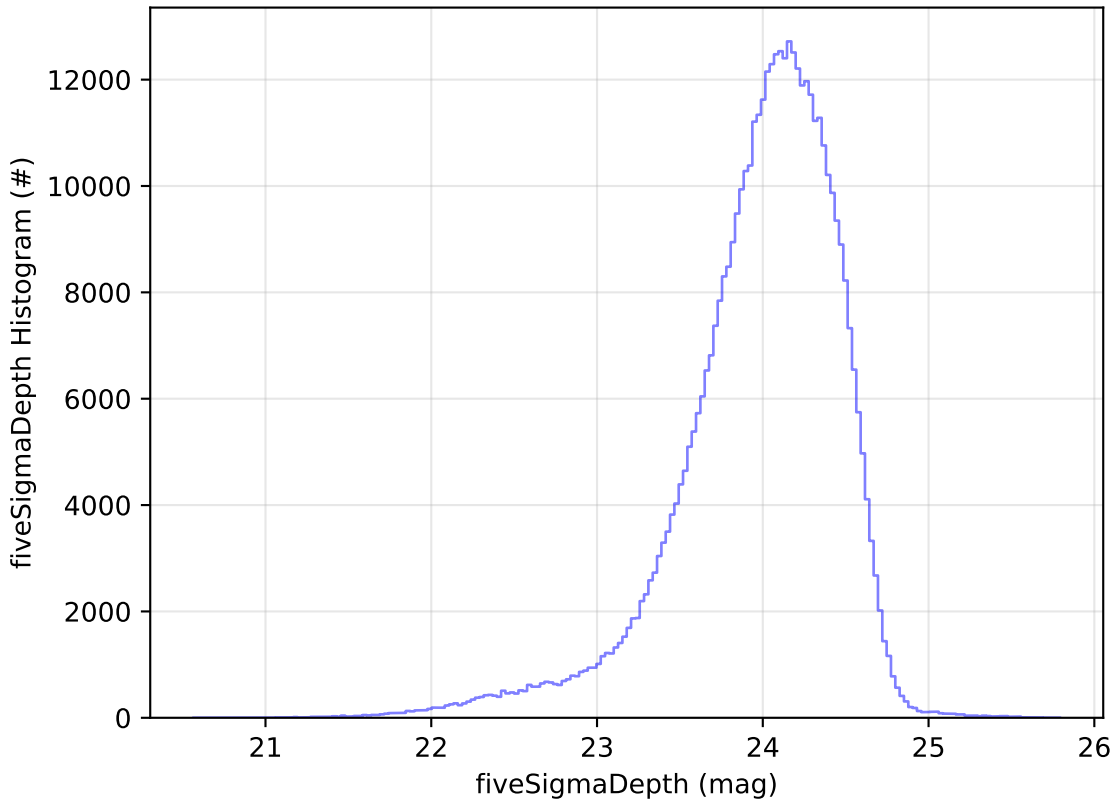
too_combined_s0.5_v3.4_10yrs WFD r band: fiveSigmaDepth Histogram
