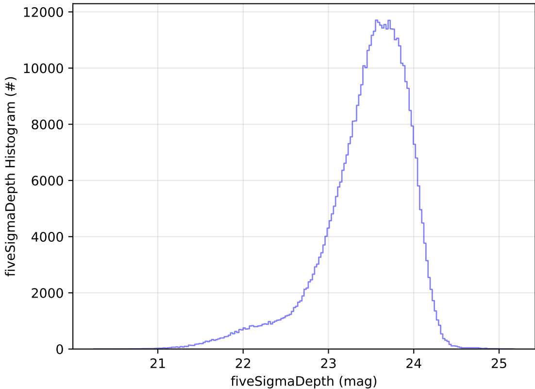
too_combined_s0.5_v3.4_10yrs WFD i band: fiveSigmaDepth Histogram
