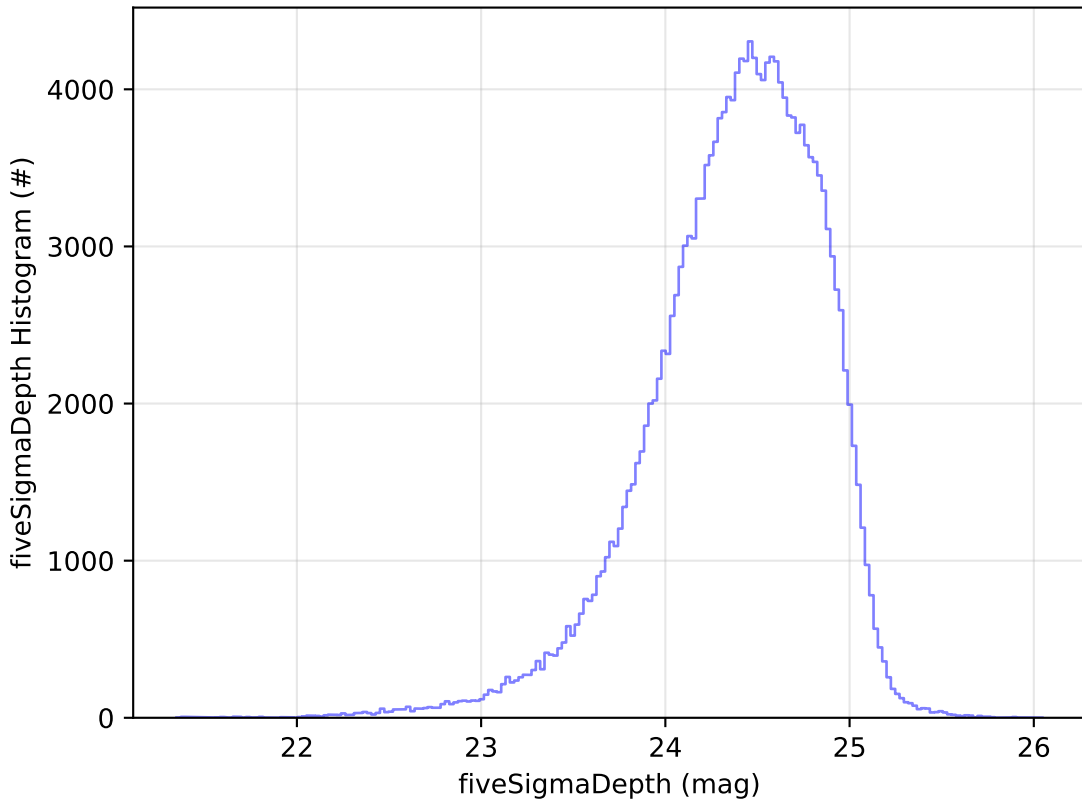
too_combined_s0.5_v3.4_10yrs WFD g band: fiveSigmaDepth Histogram
