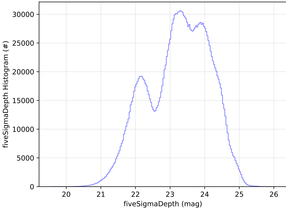
too_combined_s0.5_v3.4_10yrs WFD all bands: fiveSigmaDepth Histogram
