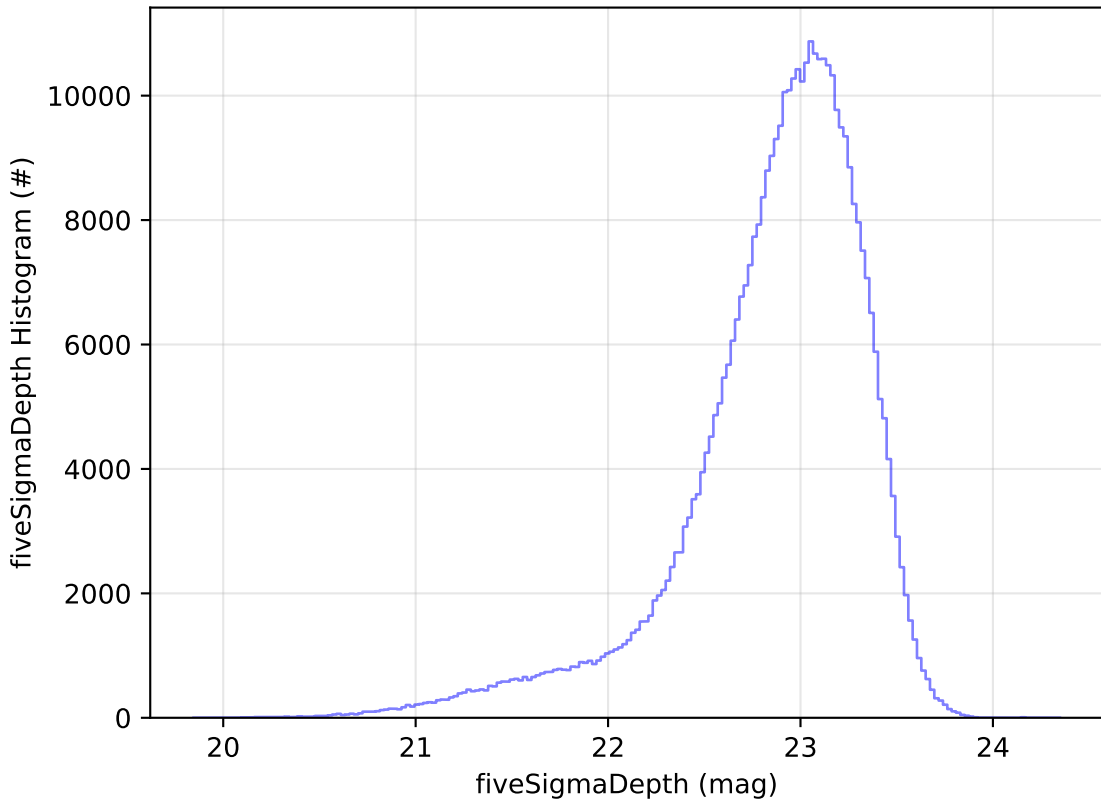
too_combined_s0.5_v3.4_10yrs All sky z band: fiveSigmaDepth Histogram
