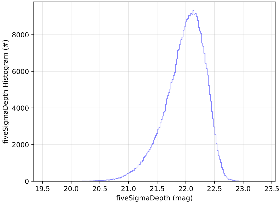
too_combined_s0.5_v3.4_10yrs All sky y band: fiveSigmaDepth Histogram
