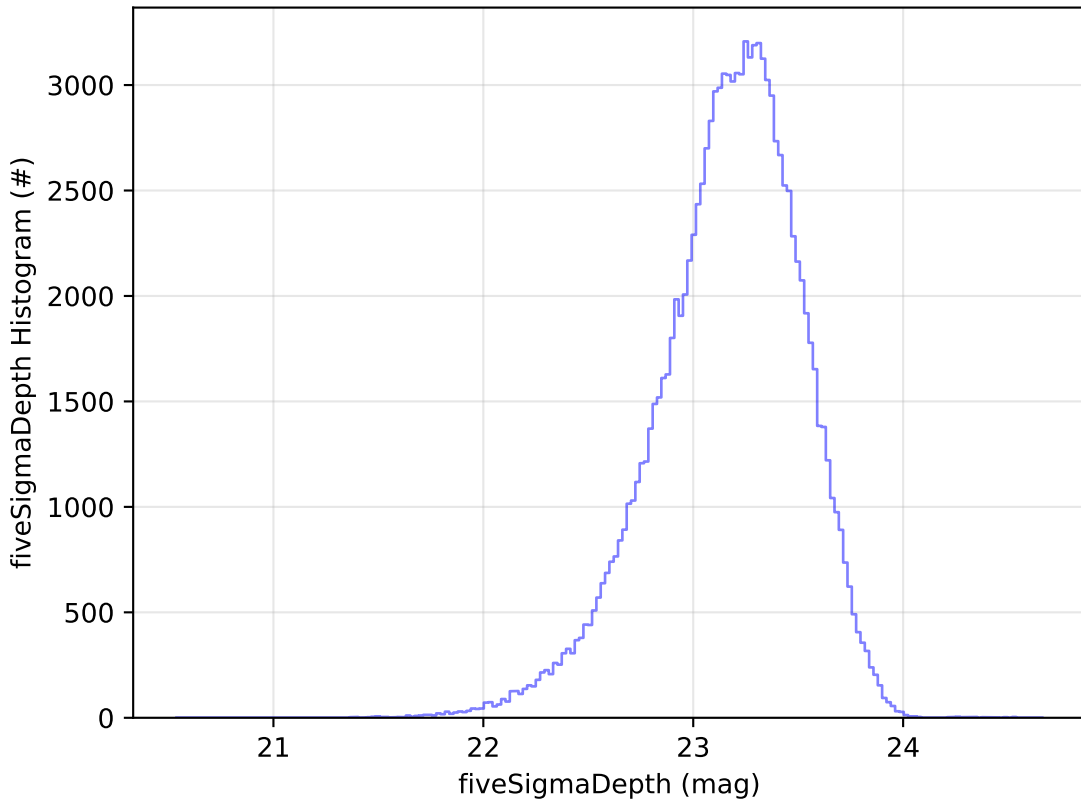
too_combined_s0.5_v3.4_10yrs All sky u band: fiveSigmaDepth Histogram
