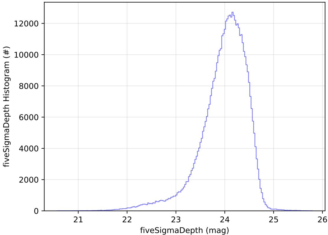
too_combined_s0.5_v3.4_10yrs All sky r band: fiveSigmaDepth Histogram
