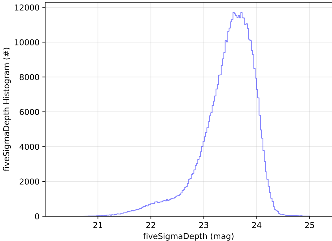
too_combined_s0.5_v3.4_10yrs All sky i band: fiveSigmaDepth Histogram
