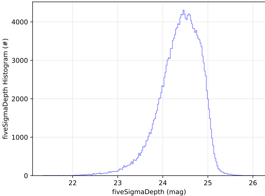
too_combined_s0.5_v3.4_10yrs All sky g band: fiveSigmaDepth Histogram
