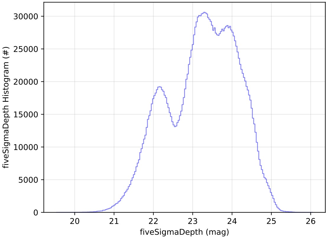
too_combined_s0.5_v3.4_10yrs All sky all bands: fiveSigmaDepth Histogram
