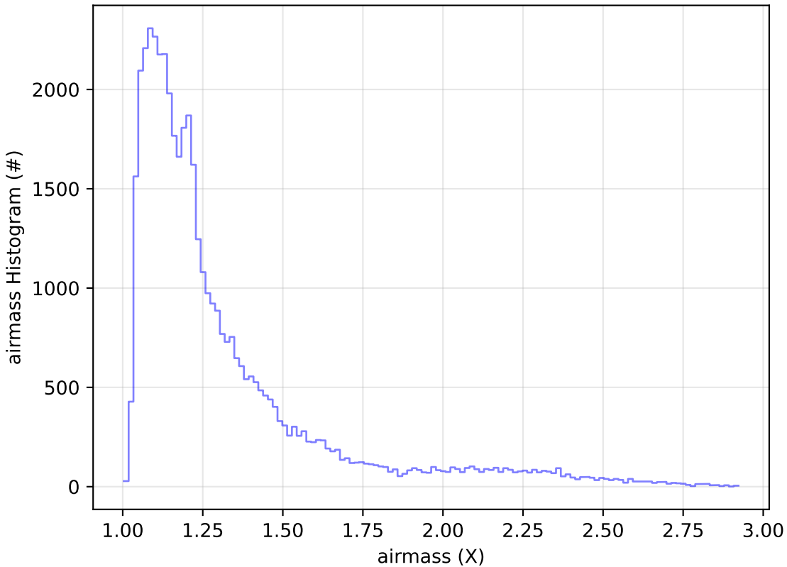
too_combined_s0.5_v3.4_10yrs Yr 1 z band: airmass Histogram
