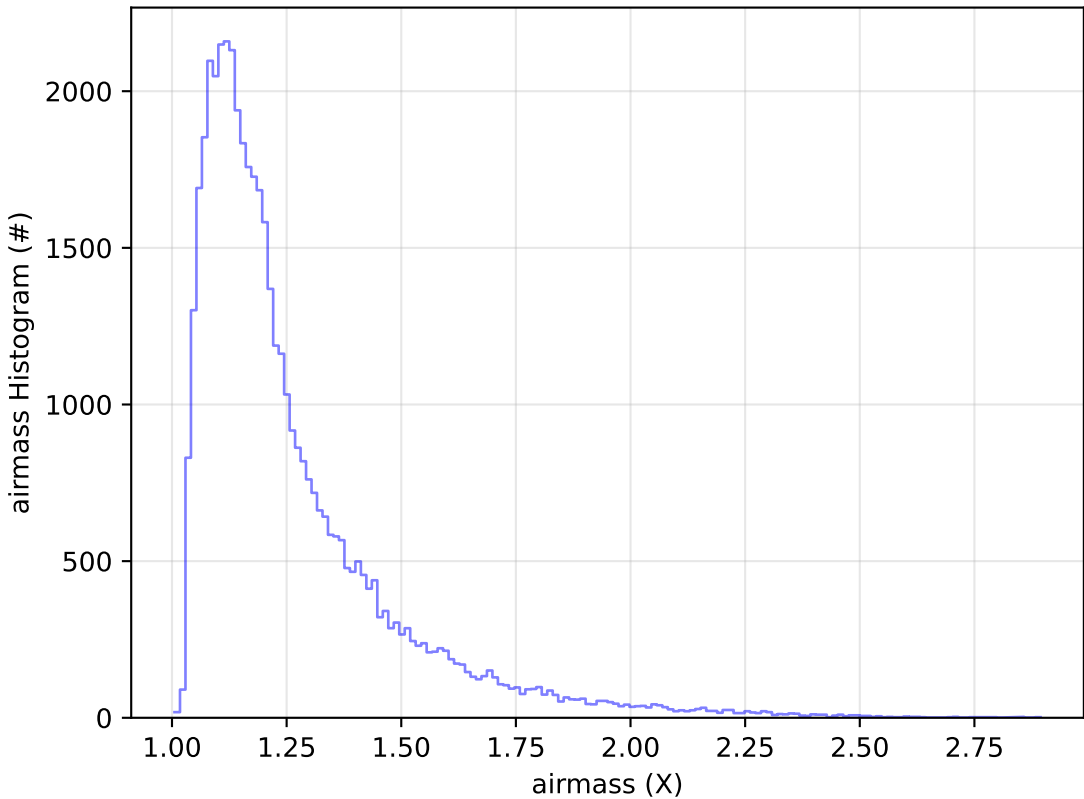
too_combined_s0.5_v3.4_10yrs Yr 1 y band: airmass Histogram
