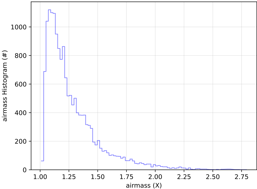
too_combined_s0.5_v3.4_10yrs Yr 1 u band: airmass Histogram
