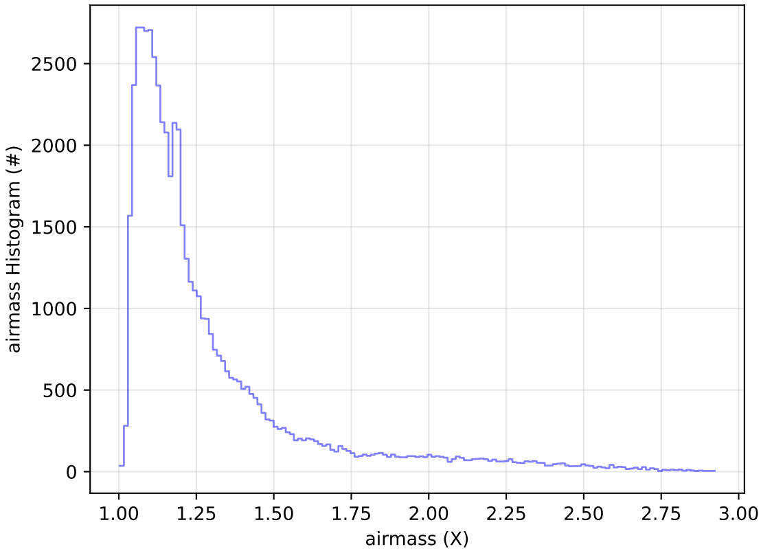
too_combined_s0.5_v3.4_10yrs Yr 1 i band: airmass Histogram
