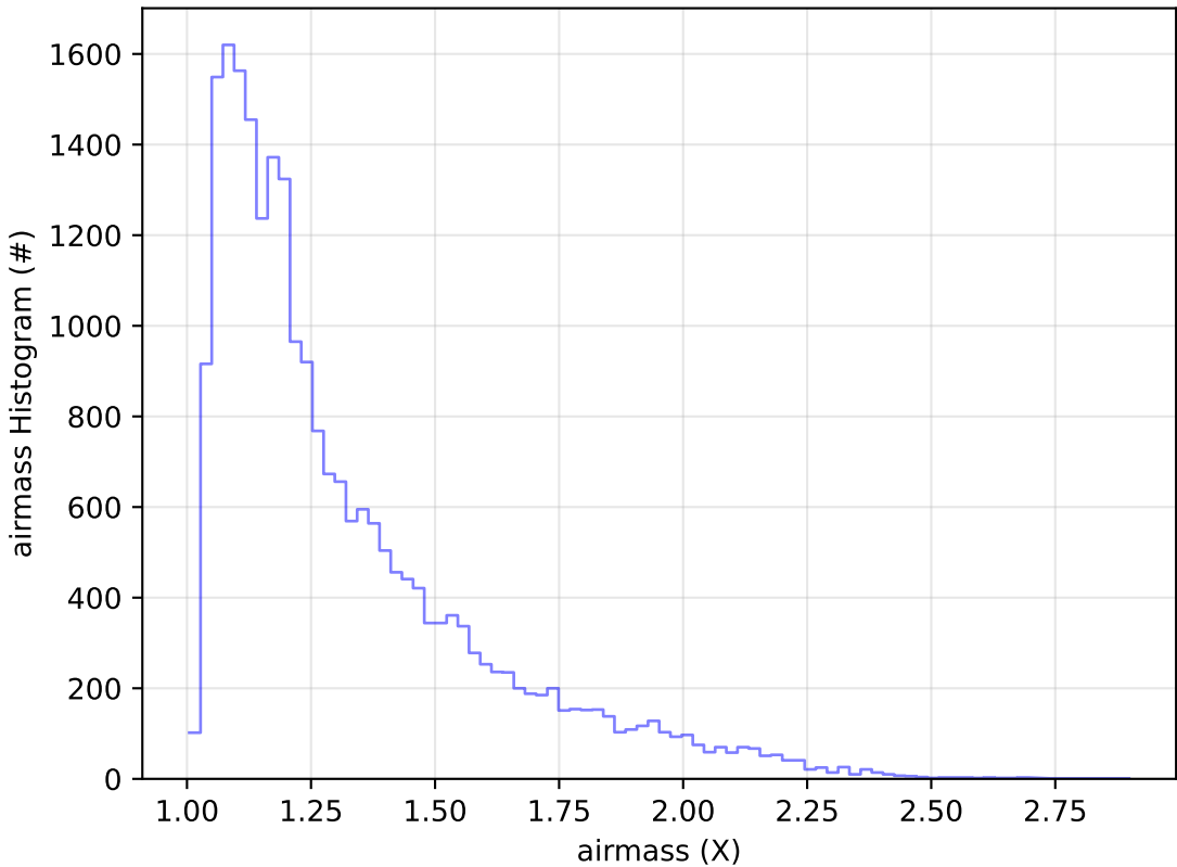
too_combined_s0.5_v3.4_10yrs Yr 1 g band: airmass Histogram
