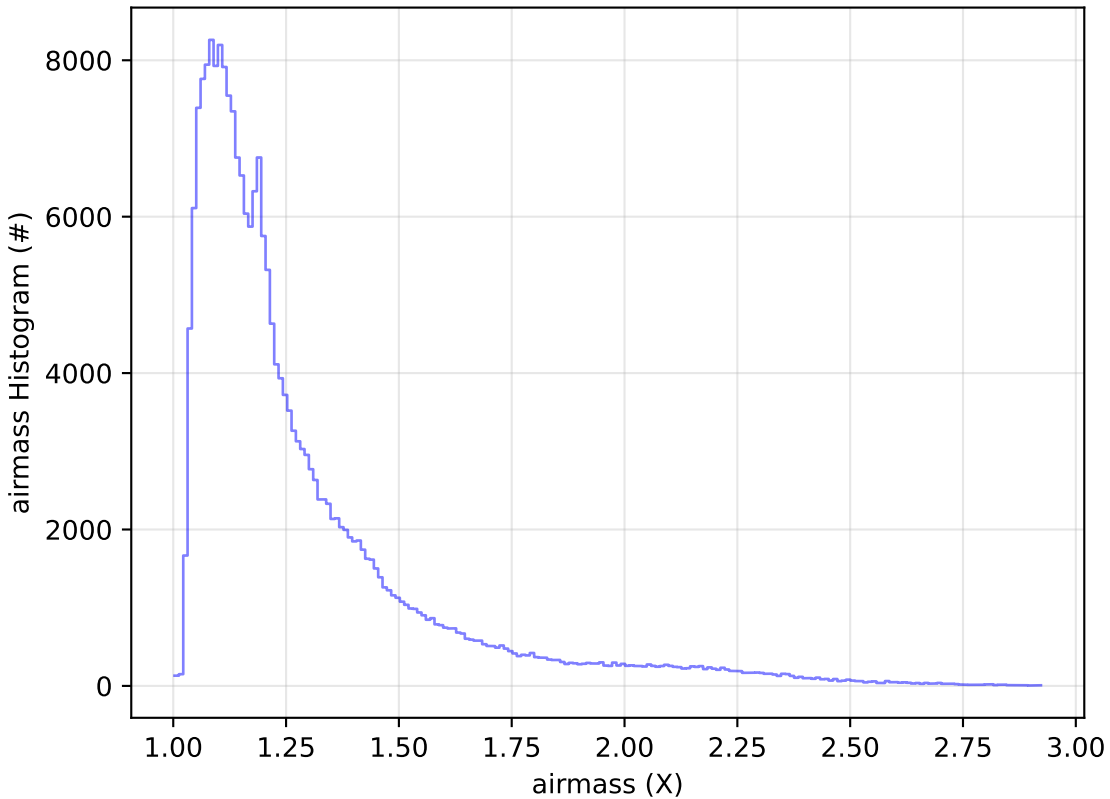
too_combined_s0.5_v3.4_10yrs Yr 1 all bands: airmass Histogram
