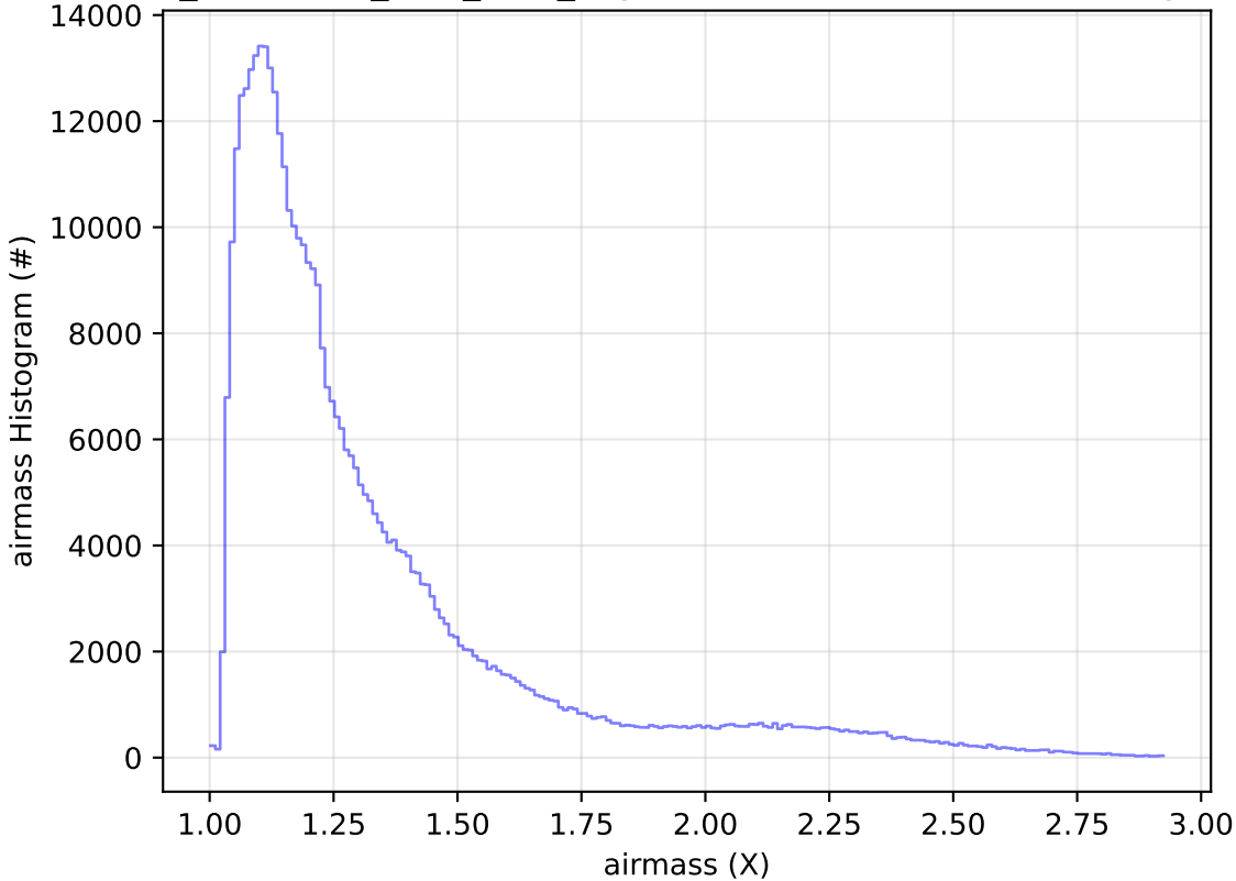
too_combined_s0.5_v3.4_10yrs WFD z band: airmass Histogram
