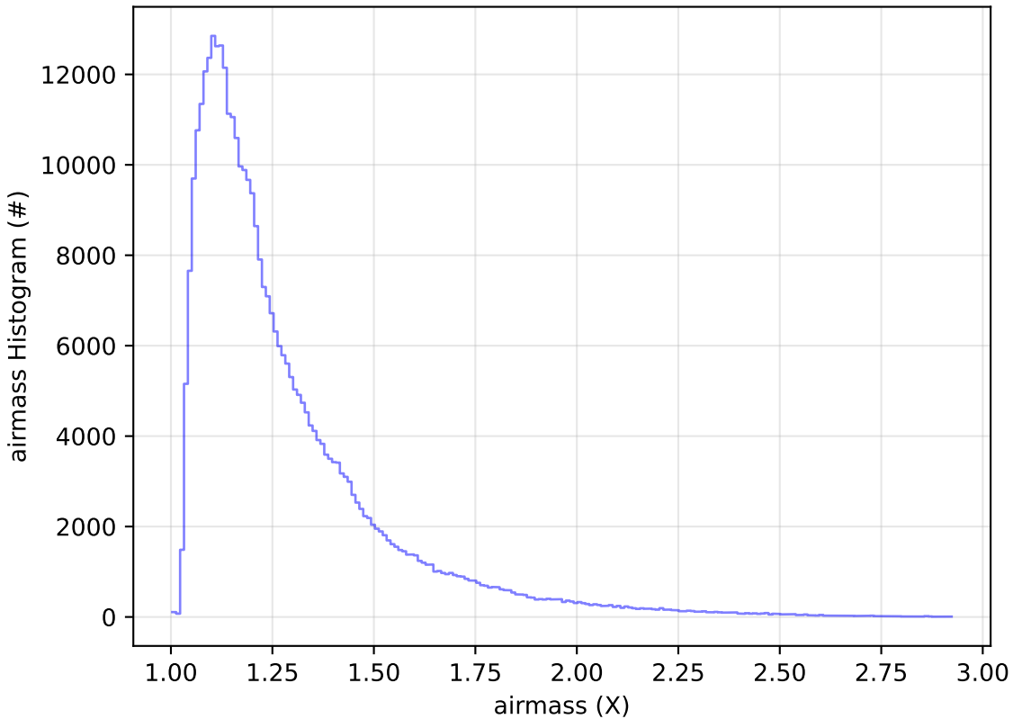
too_combined_s0.5_v3.4_10yrs WFD y band: airmass Histogram
