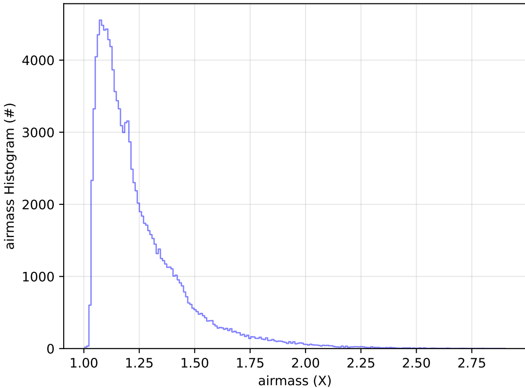
too_combined_s0.5_v3.4_10yrs WFD u band: airmass Histogram
