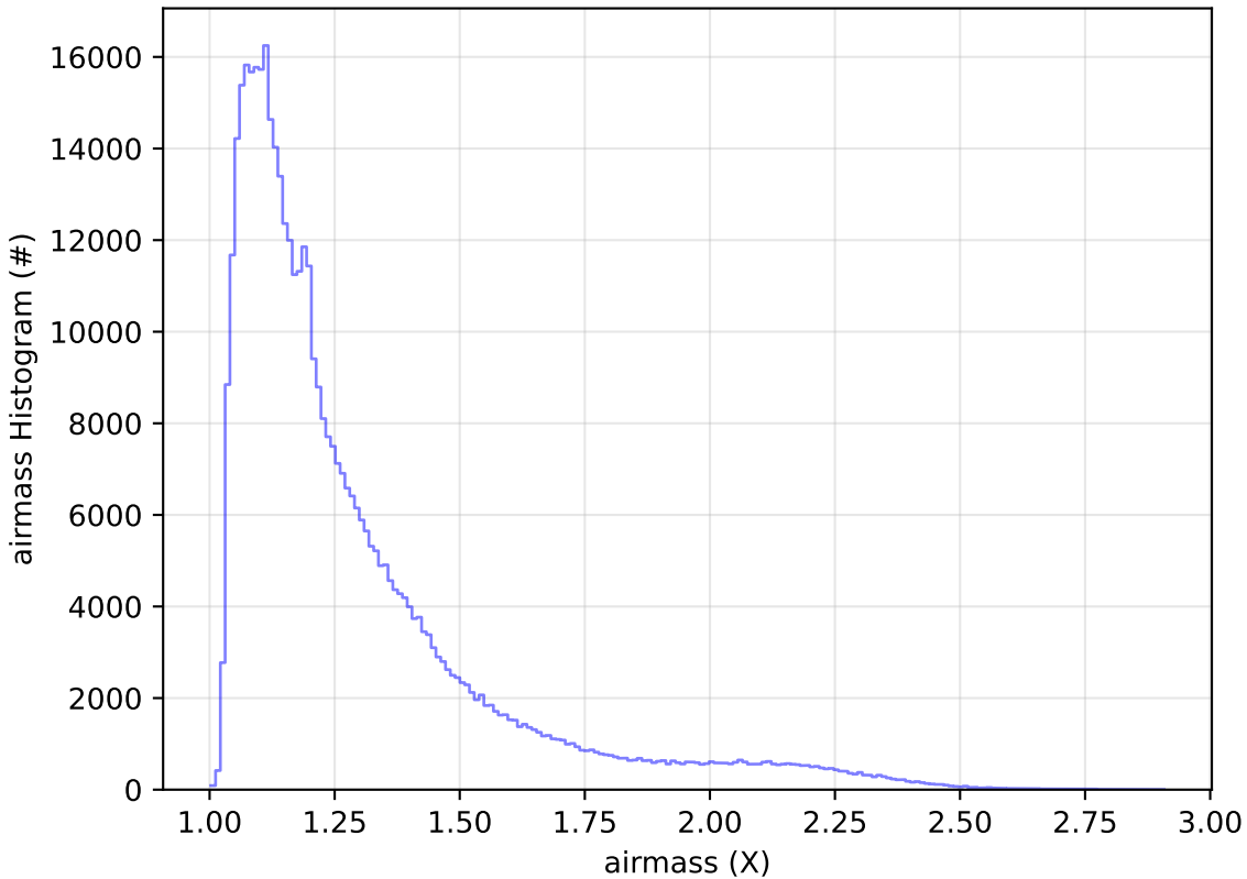
too_combined_s0.5_v3.4_10yrs WFD r band: airmass Histogram
