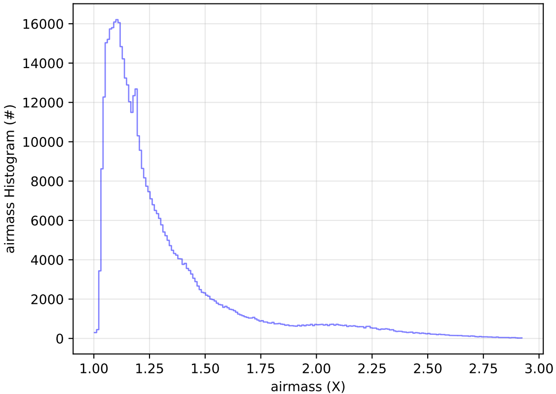
too_combined_s0.5_v3.4_10yrs WFD i band: airmass Histogram
