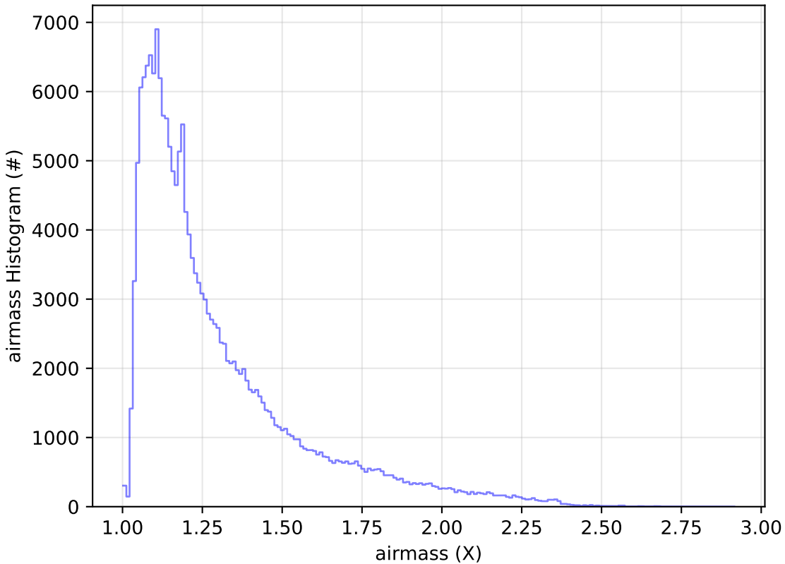
too_combined_s0.5_v3.4_10yrs WFD g band: airmass Histogram
