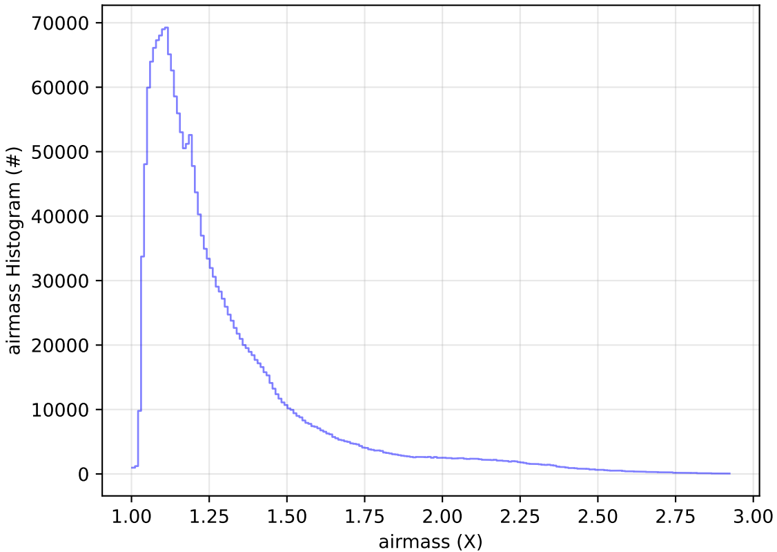
too_combined_s0.5_v3.4_10yrs WFD all bands: airmass Histogram
