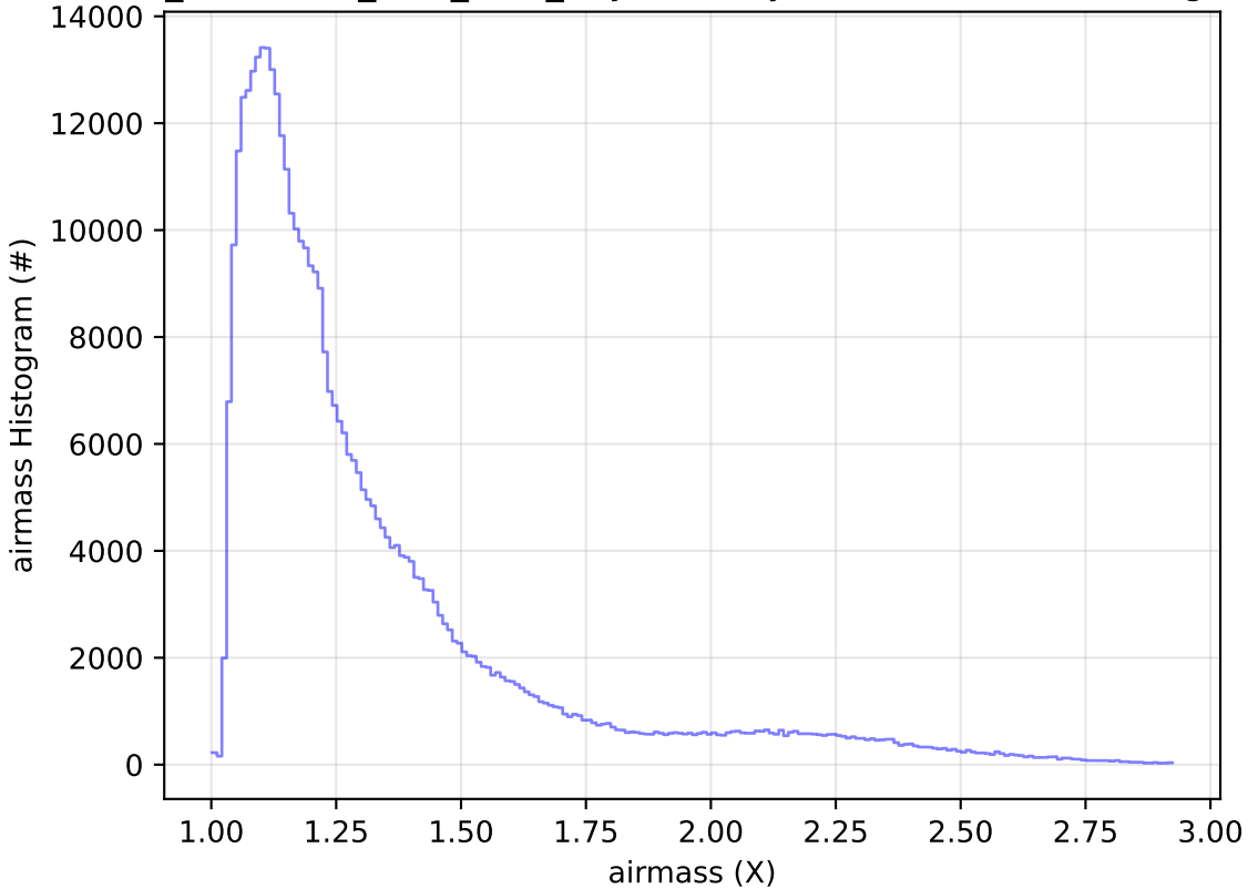
too_combined_s0.5_v3.4_10yrs All sky z band: airmass Histogram
