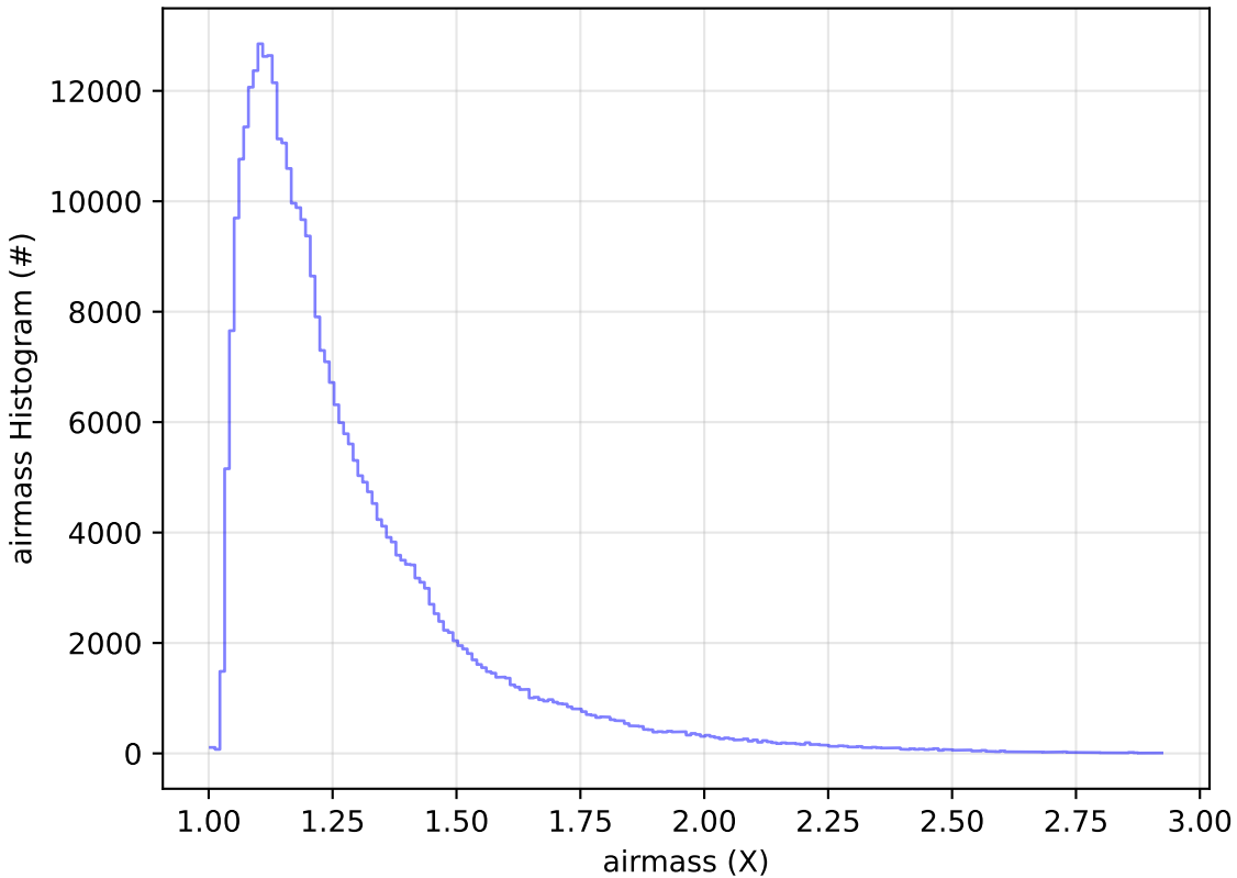
too_combined_s0.5_v3.4_10yrs All sky y band: airmass Histogram
