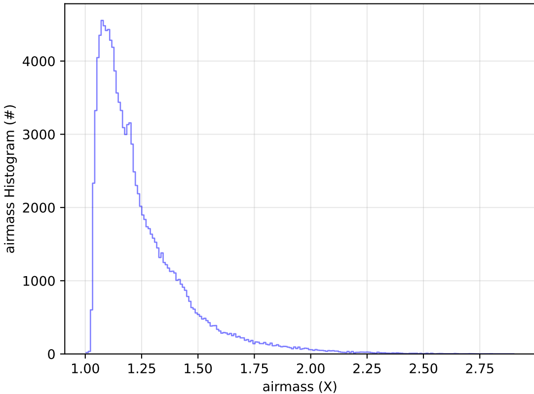
too_combined_s0.5_v3.4_10yrs All sky u band: airmass Histogram
