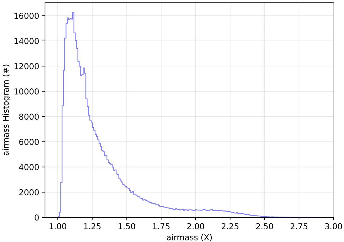
too_combined_s0.5_v3.4_10yrs All sky r band: airmass Histogram
