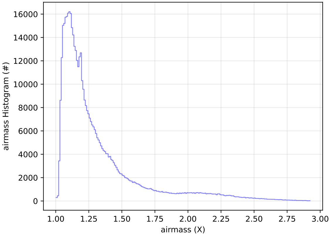
too_combined_s0.5_v3.4_10yrs All sky i band: airmass Histogram
