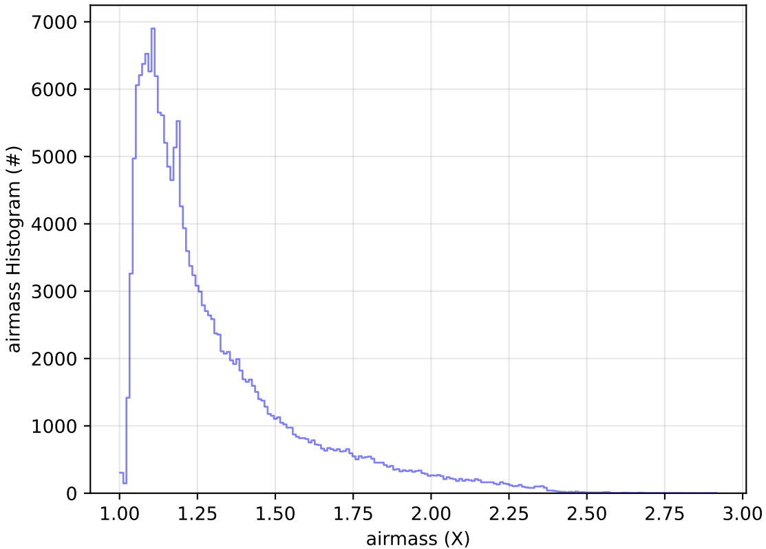
too_combined_s0.5_v3.4_10yrs All sky g band: airmass Histogram
