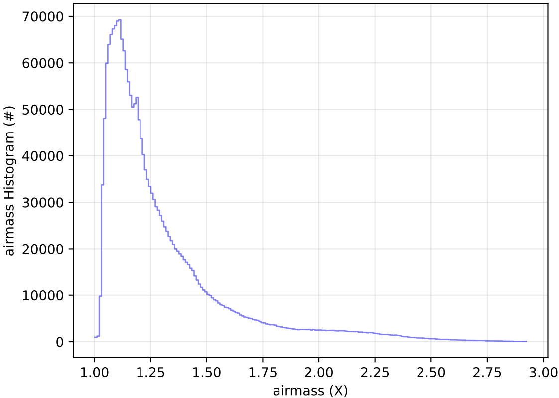
too_combined_s0.5_v3.4_10yrs All sky all bands: airmass Histogram
