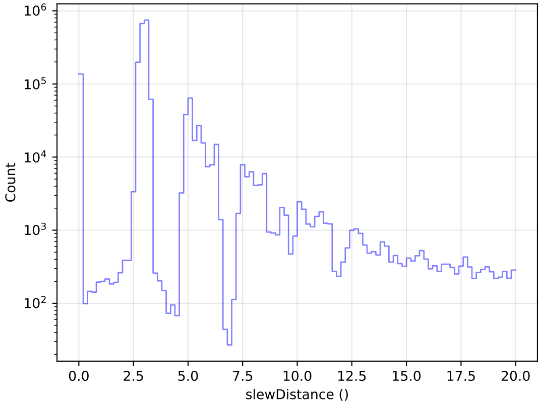
too_combined_s0.5_v3.4_10yrs All visits: Zoom Slew Distance Histogram
