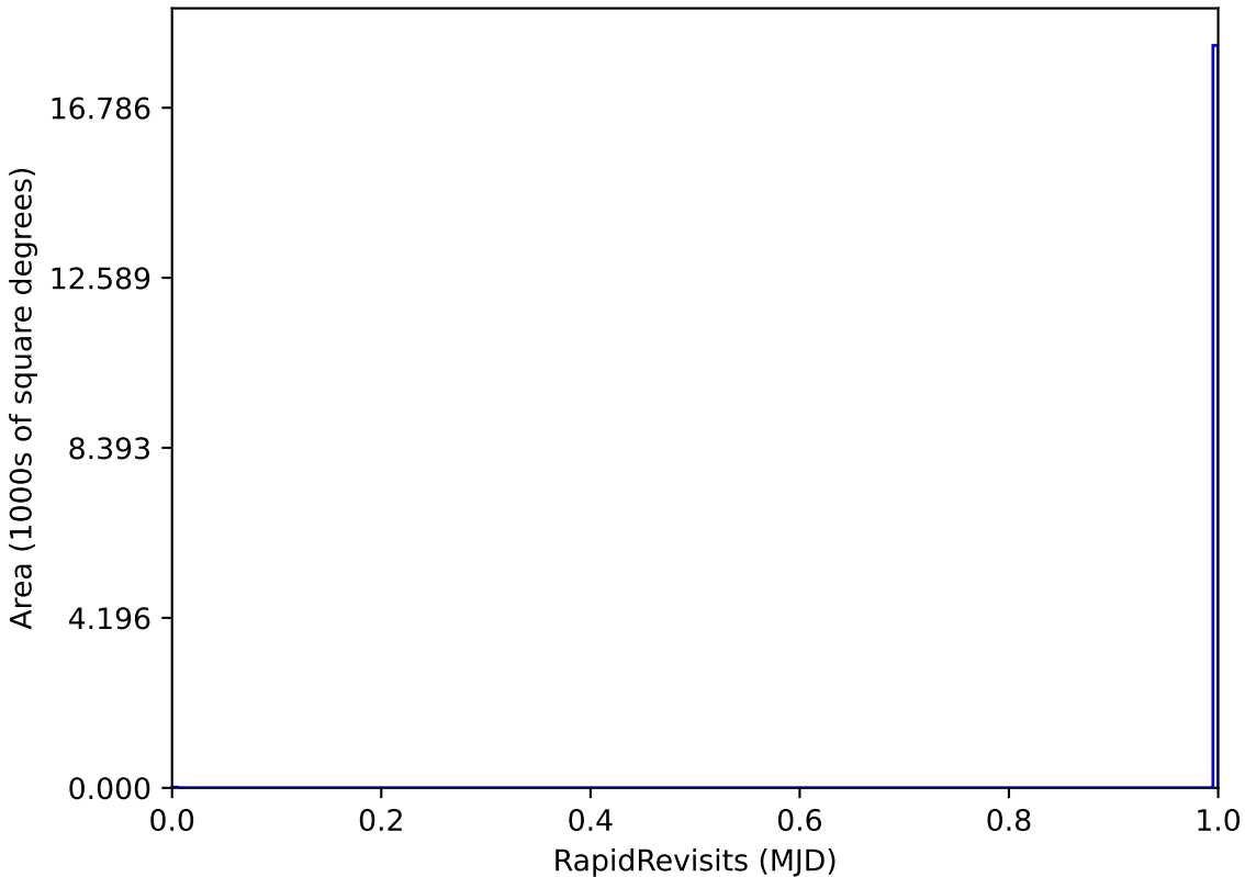
too_combined_s0.5_v3.4_10yrs WFD: RapidRevisits
