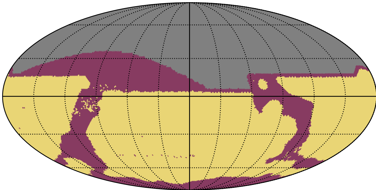
too_combined_s0.5_v3.4_10yrs All sky: RapidRevisits
