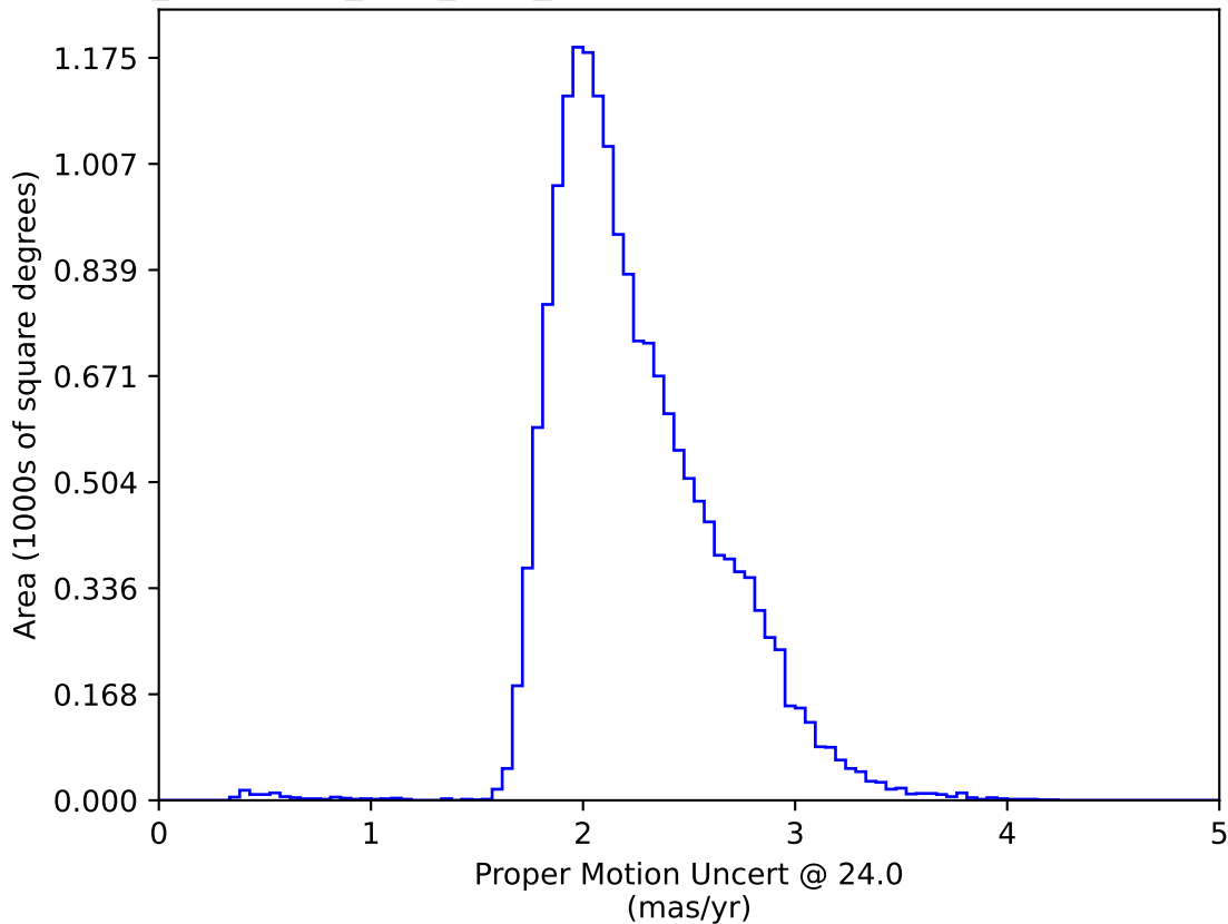
too_combined_s0.5_v3.4_10yrs WFD: Proper Motion Uncert @ 24.0
